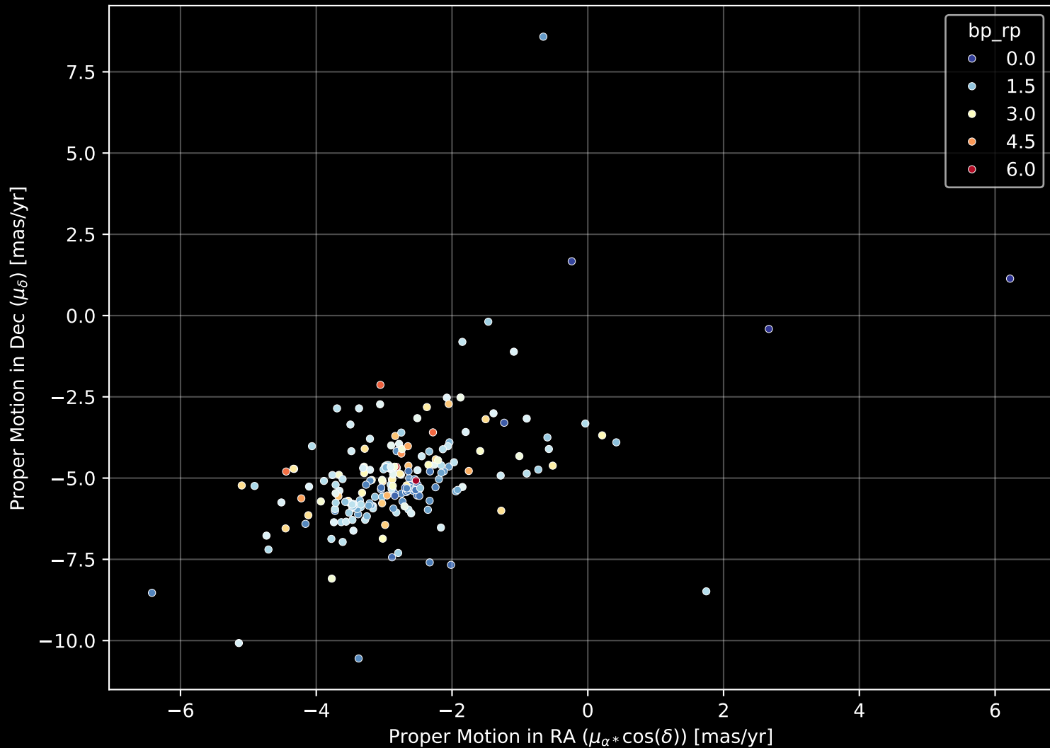
APOGEE DR17 Field: [FL_2020] Proper Motion Diagram (n= 208)
