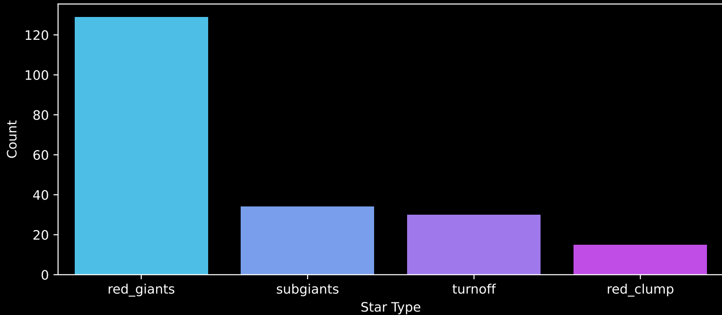
APOGEE DR17 Field: [FL_2020] Count plot of Star Type
