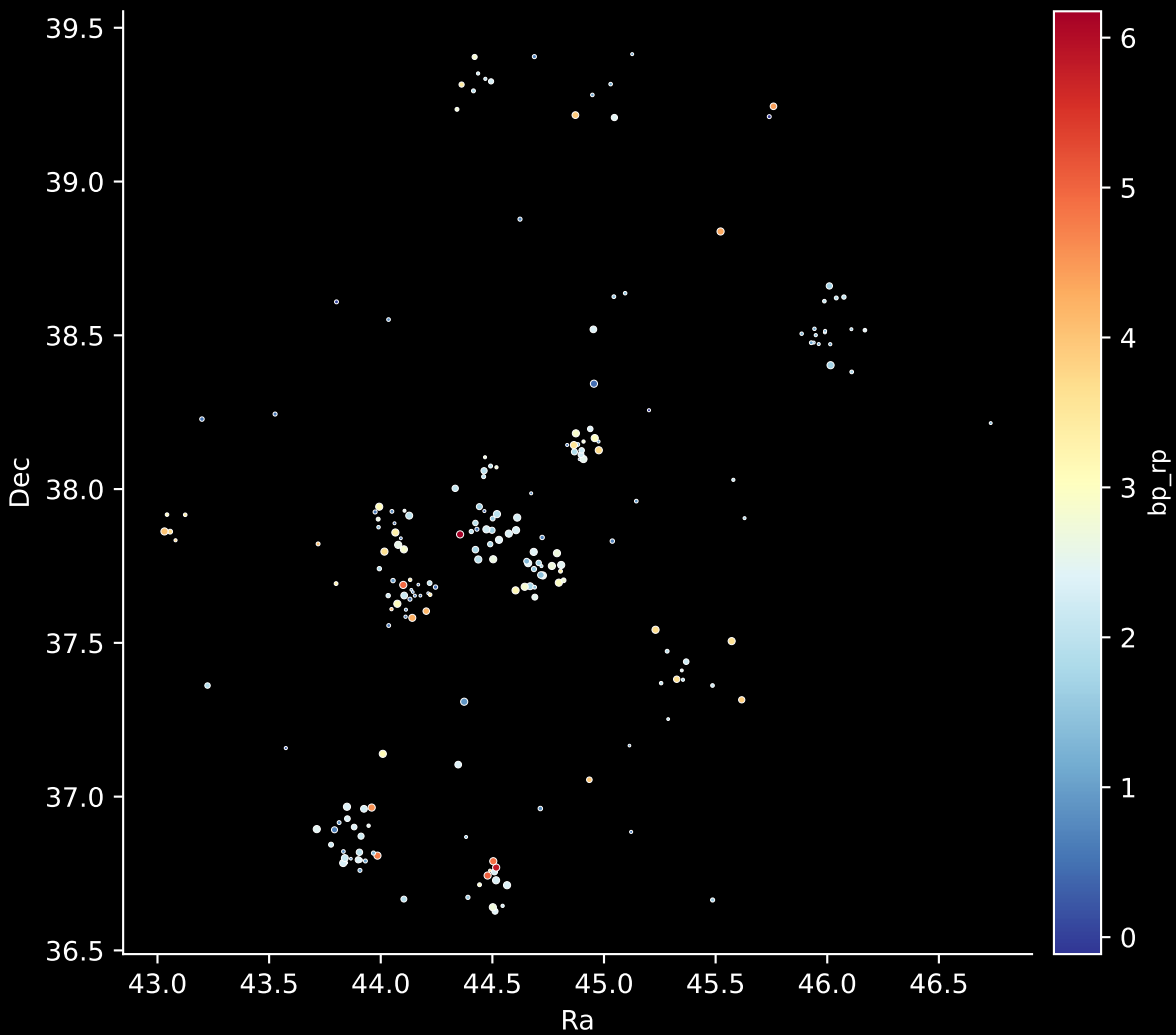
APOGEE DR17 Field: [FL_2020] Stars: 208
