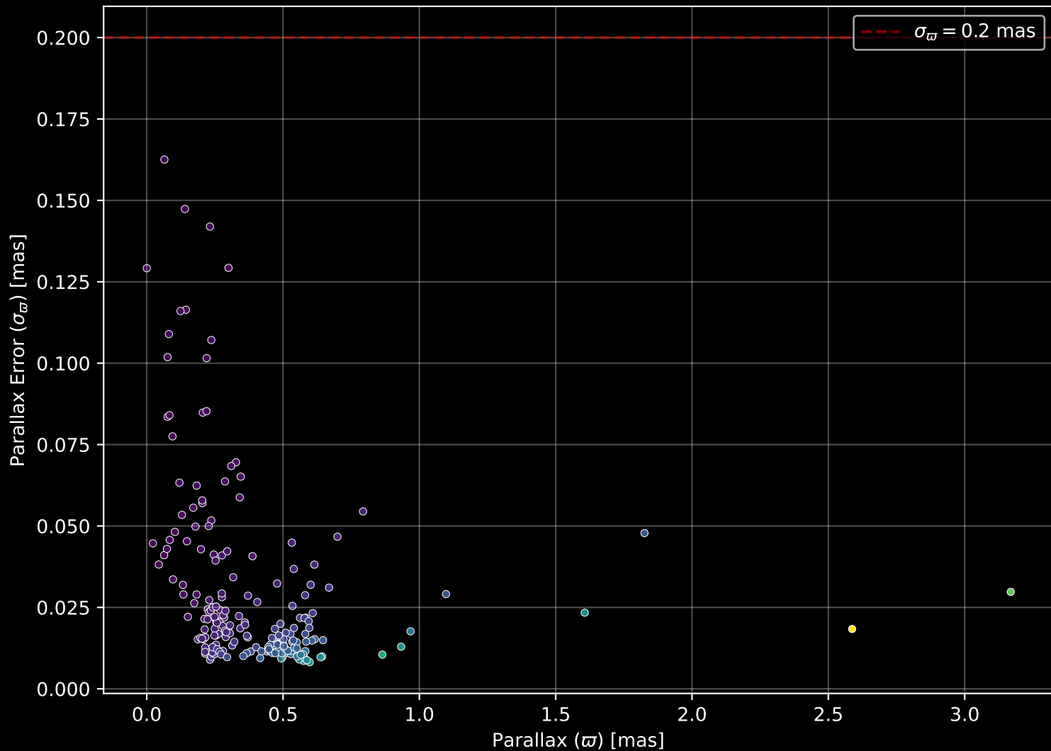
APOGEE DR17 Field: [FL_2020] Parallax Quality (n= 208)
