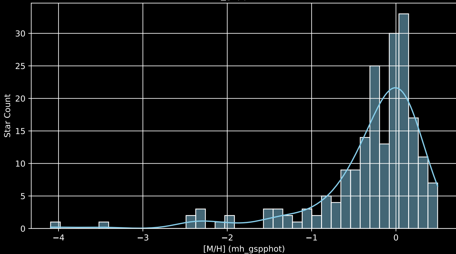
APOGEE DR17 Field: [FL_2020 [M/H] (mh_gspphot) (n= 201)
