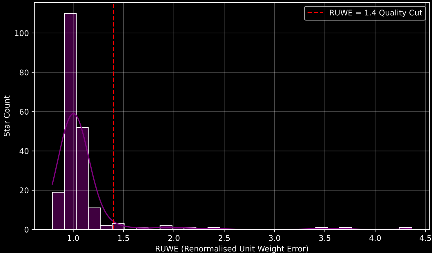
GAPOGEE DR17 Field [FL_2020] RUWE Distribution (n= 206)
